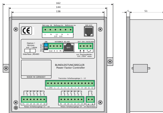
Dimensions Dimensional drawing PFC-12TR-1/PFC-12TR-1-RS485
