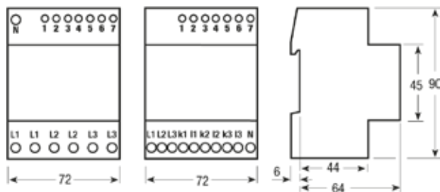
Dimensional drawing
