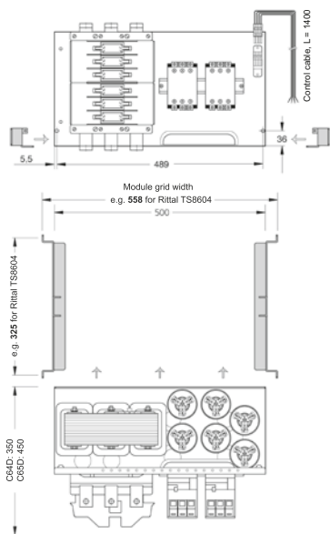
Dimensional drawing type series C64D (25 to 100 kvar) with module rails (here: MT-C6-Rittal VX 8604)
