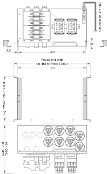
Dimensional drawing type series C64C (25 to 100 kvar) with module rails (here: MT-C6-Rittal VX 8604)
