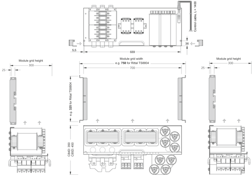
Dimensional drawing type series C84D (25 to 100 kvar) with module rails (here: MT-C8-Rittal VX 8804)
