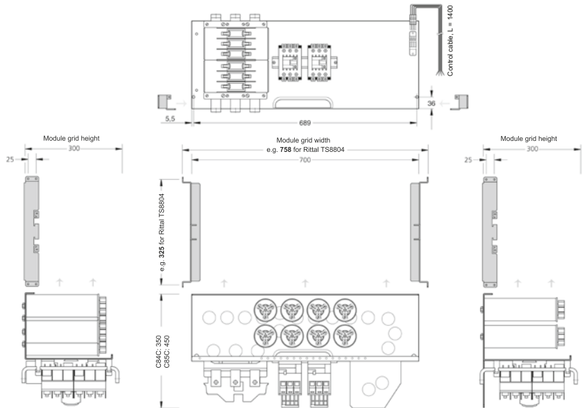
Dimensional drawing type series C84C (25 to 100 kvar) with module rails (here: MT-C8-Rittal VX 8804)
