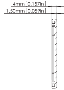
SECTION C-C SCALE 1 : 1
