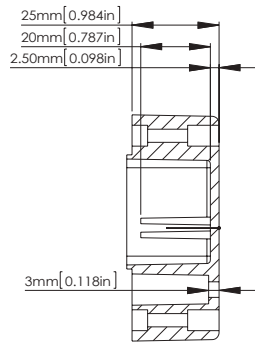
SECTION A-A FOUR (4) M4X20 mm FLAT HEAD SCREWS
