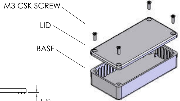
ISO VIEW
