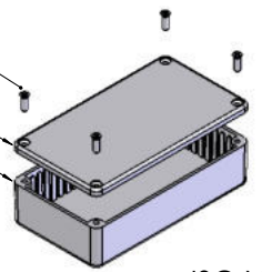
ISO VIEW 1:3
