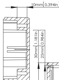
SECTION B-B
