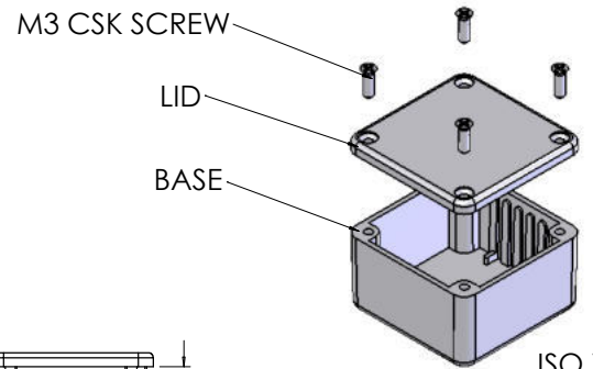
ISO VIEW 1:2
