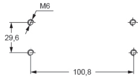
Catalogue drawings
