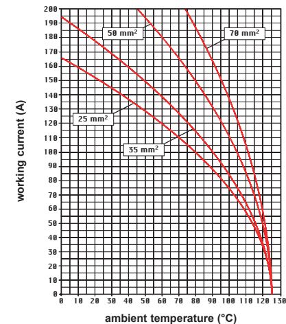
CX 01 YA, 1 pole connector inserts (MIXO 200A) Maximum current load derating diagram
