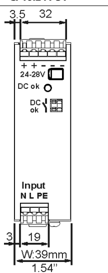
Fig. 20-2 Front view CP10.241-S1
