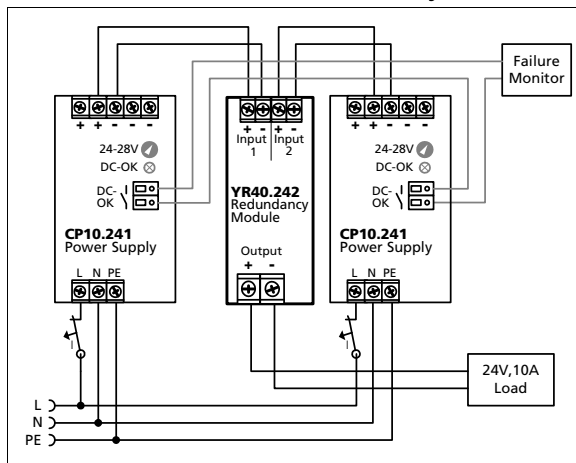
Fig. 21-1 Typical 1+1 Redundant configuration for 10A with the YR40.242 MOSFET redundancy module
