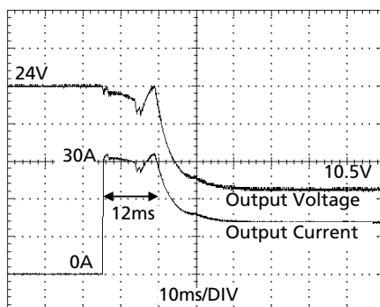
Fig. 22-3 30A Peak load, typ.
