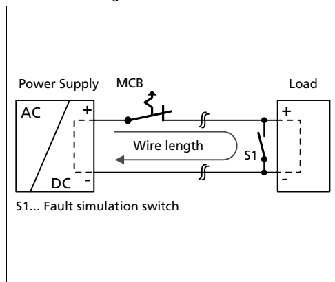
Fig. 22-4 Test circuit
