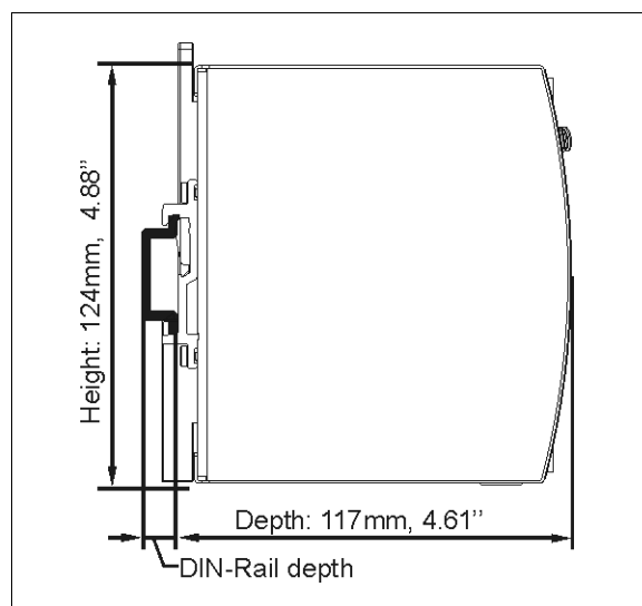
Fig. 20-3 Side view
