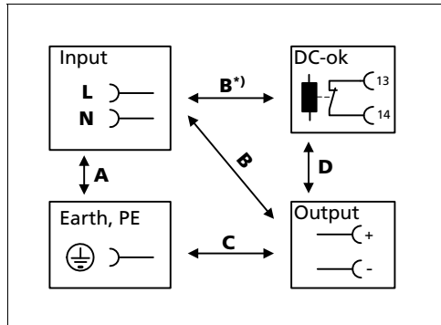
Fig. 18-1 Dielectric strength
