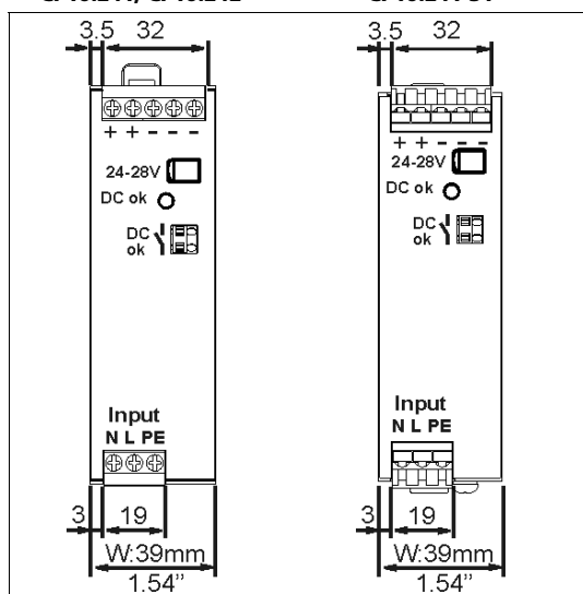
Fig. 20-1 Front view CP10.241, CP10.242
