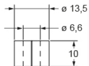
Catalogue drawings
