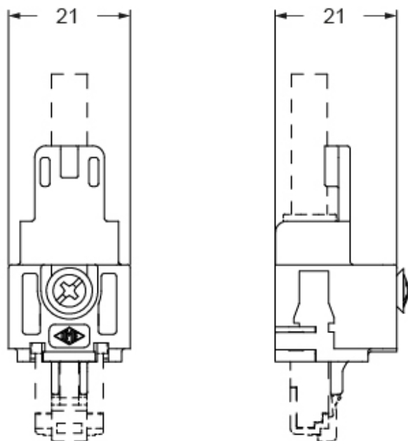
Catalogue drawings
