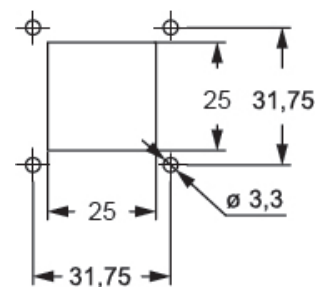
Catalogue drawings
