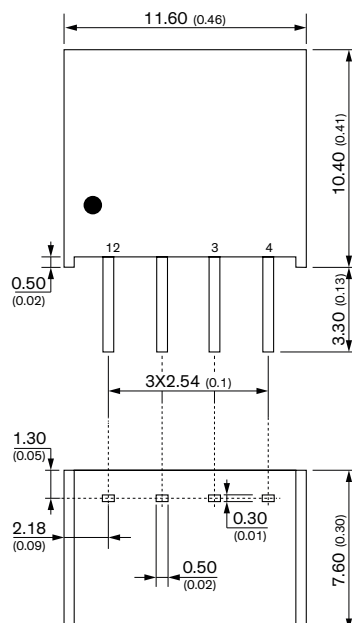
Pinout
