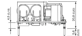
3, 3, 5, and 9 VDC models - with heatsink
